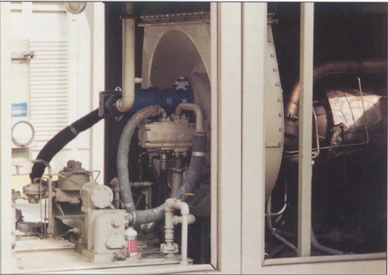
56S mounted on a Solar Saturn Engine.
