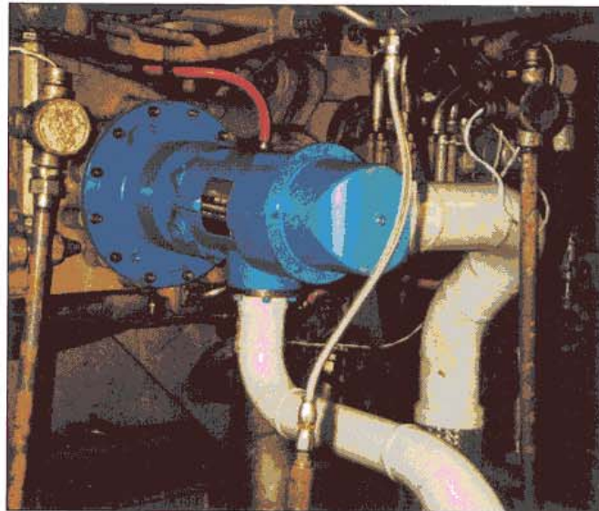
56G mounted on a GE LM2500 Engine.
