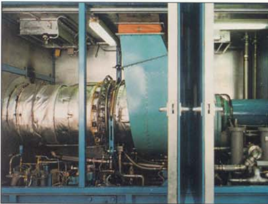
56B mounted on a DR 990 Gen Set package.
